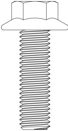
M8 x 1.25mm x 25mm Hex Head
